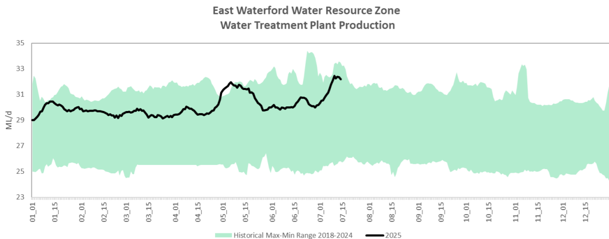
Figure 15 - East Waterford Water Resource Zone water Treatment Plant Production compared to historical Max-Min values.
