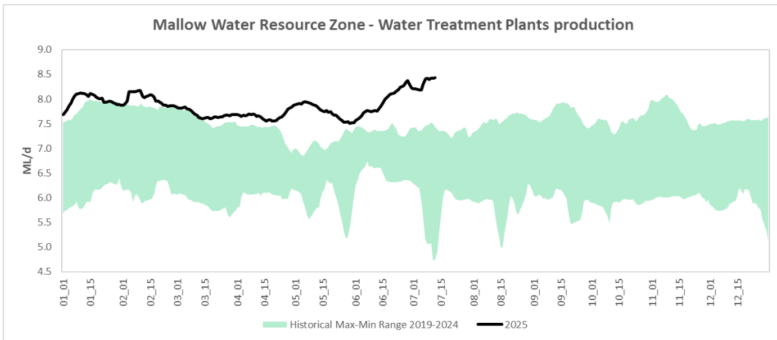
Figure 13 - Mallow Water Resource Zone water Treatment Plant Production compared to historical Max-Min values.
