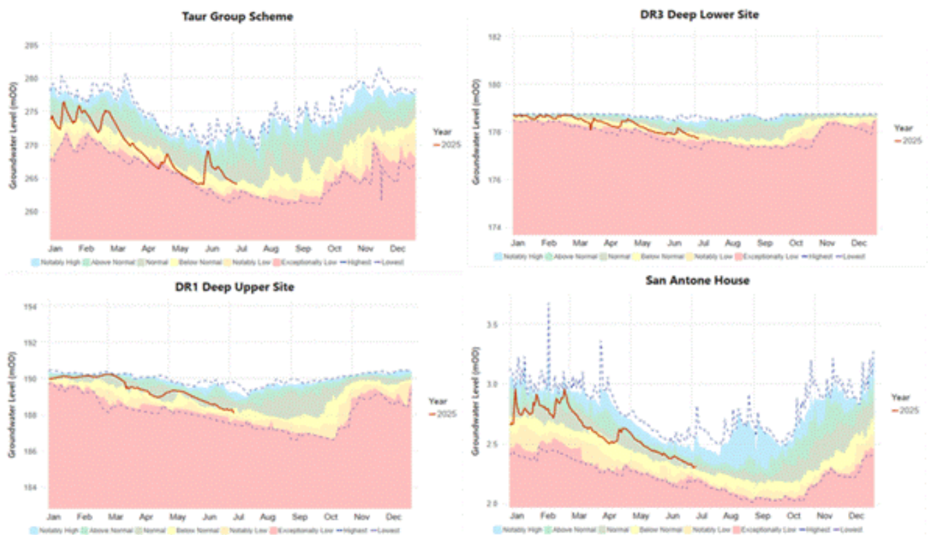
Figure 11: Daily groundwater levels recorded in 2025 at the Taur Group Scheme, DR1 Deep Upper Site, DR3 Deep Lower Site and San Antone House EPA gauges shown relative to historic daily values expressed as percentiles of all years on record - namely: 5th, 15th, 35th, 65th, 85th and 95th.
