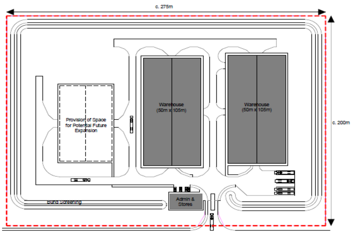
Indicative layout of proposed Regional Biosolids Storage Facility
