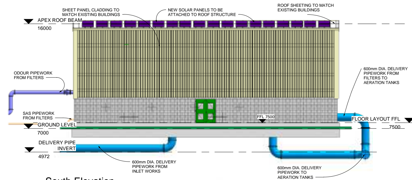
4 South Elevation 1 : 100
