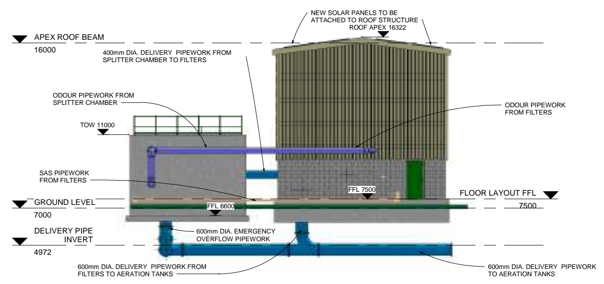
3 West Elevation 1 : 100
