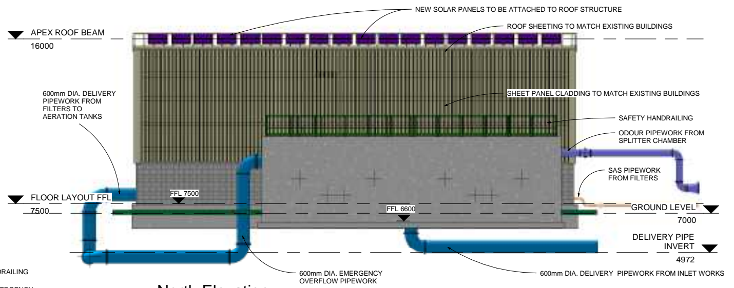
2 North Elevation 1 : 100
