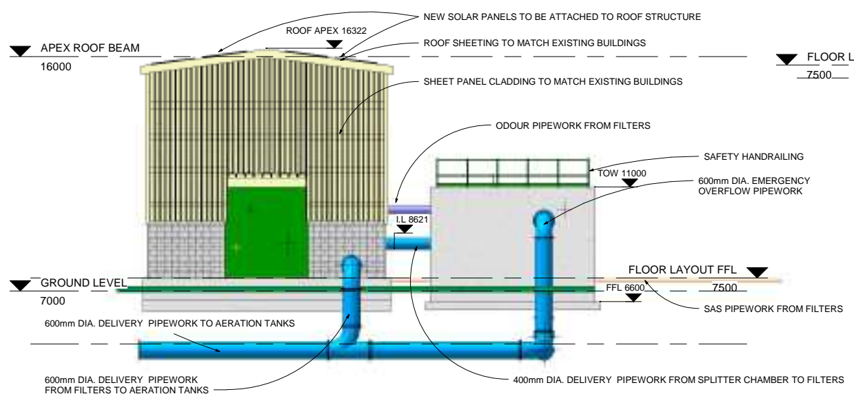
1 East Elevation 1 : 100
