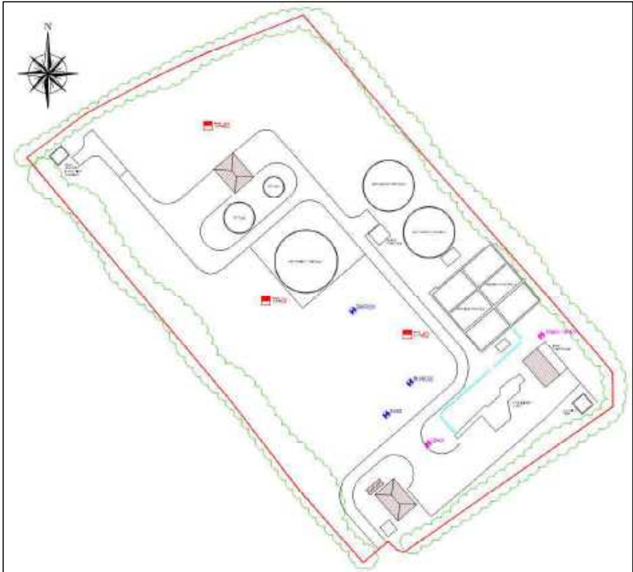
Figure 13-2: Ground Investigation Layout Plan
