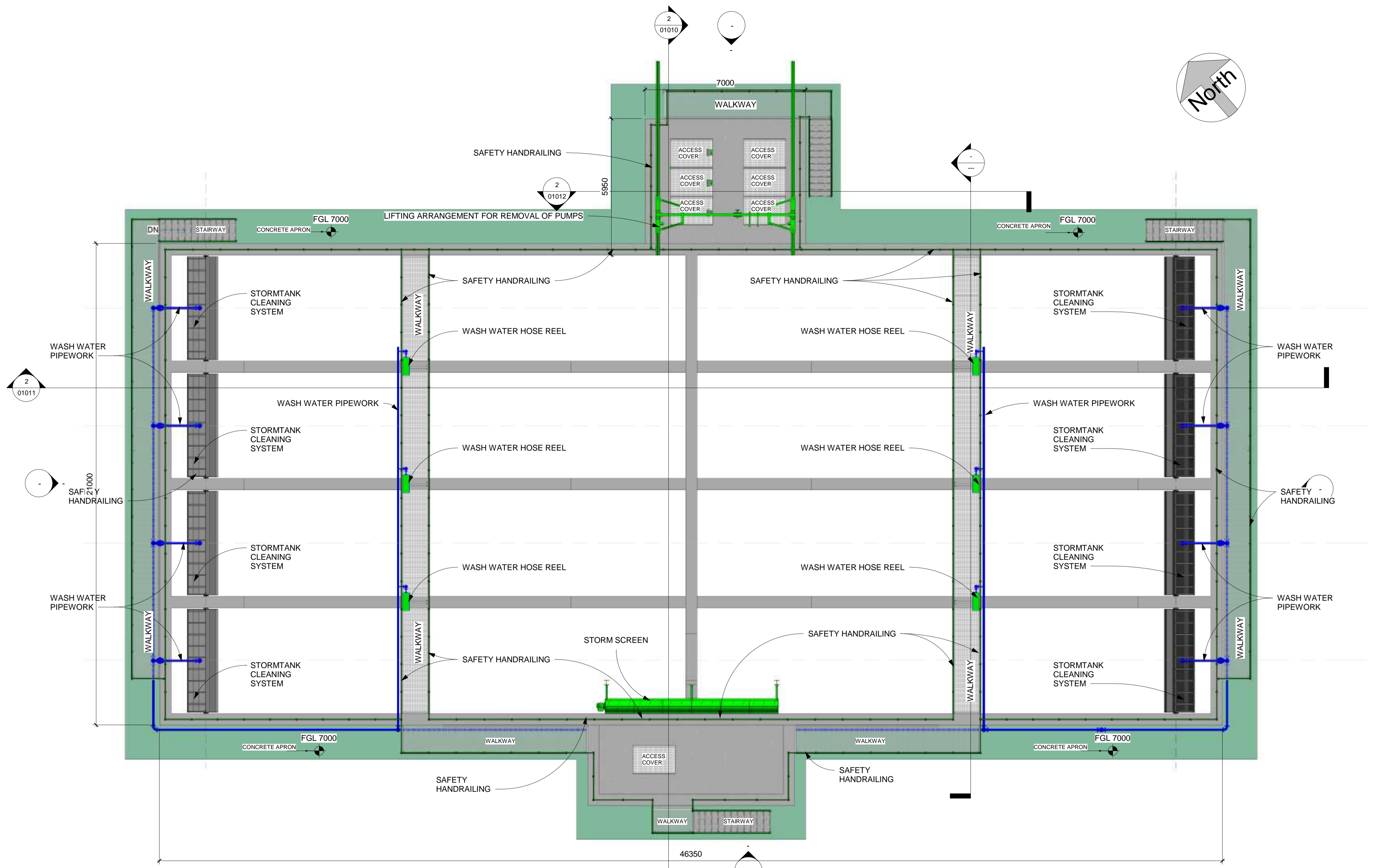
1 TOW - Stormwater Storage Tank 1 : 100
