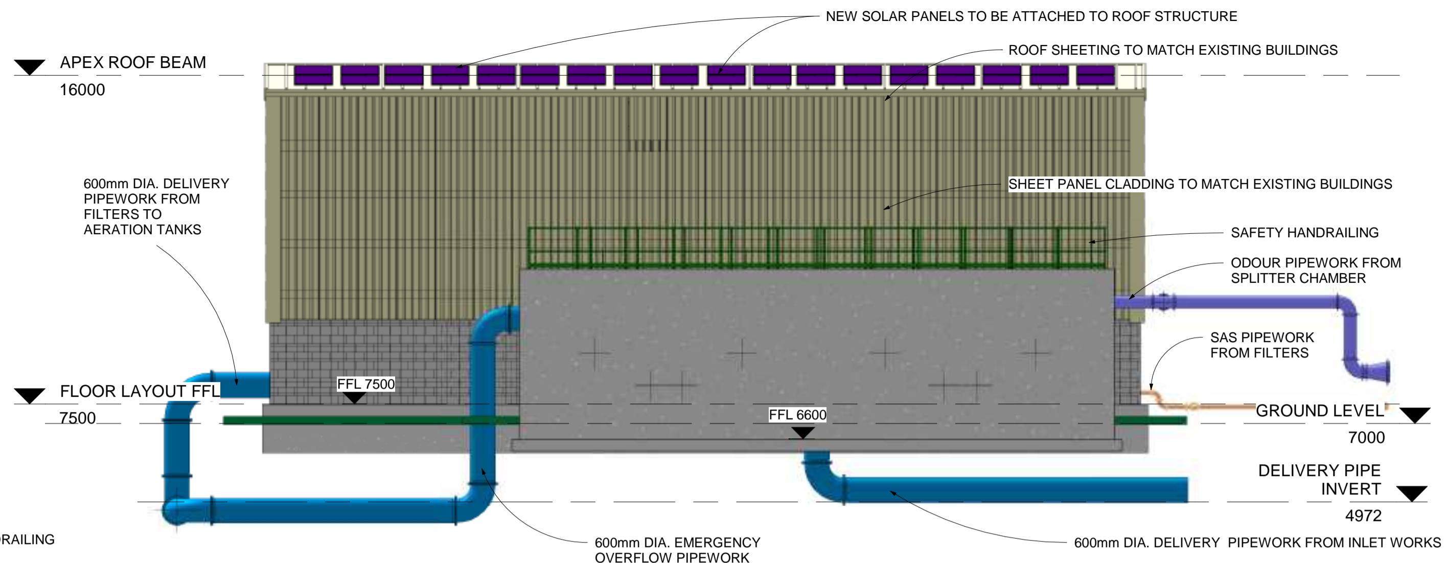
2 North Elevation 1 : 100
