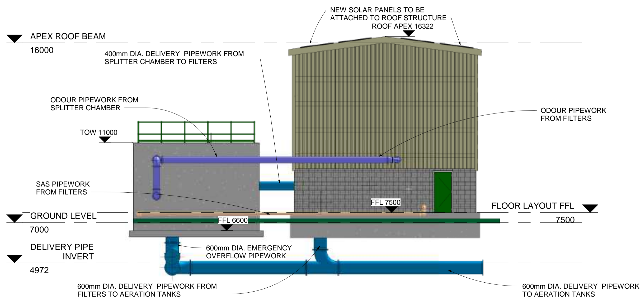
3 West Elevation 1 : 100
