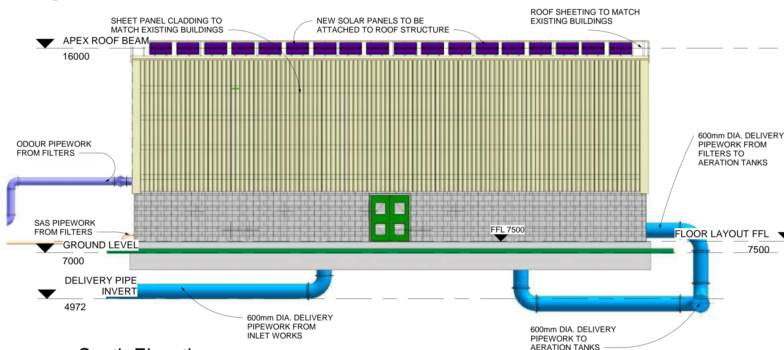
4 South Elevation 1 : 100
