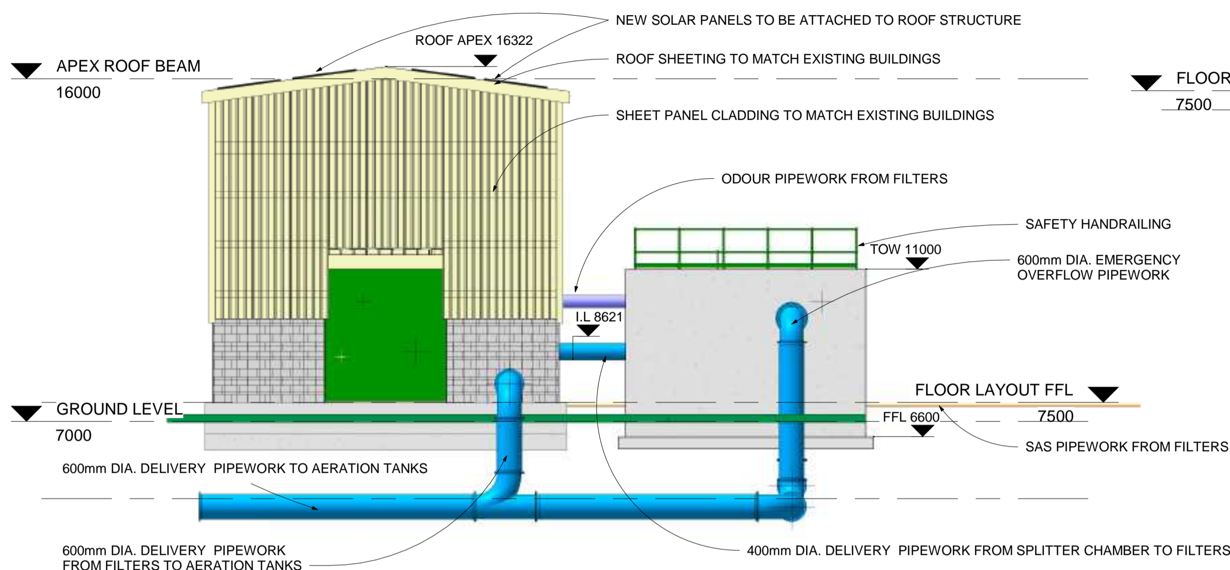
1 East Elevation 1 : 100
